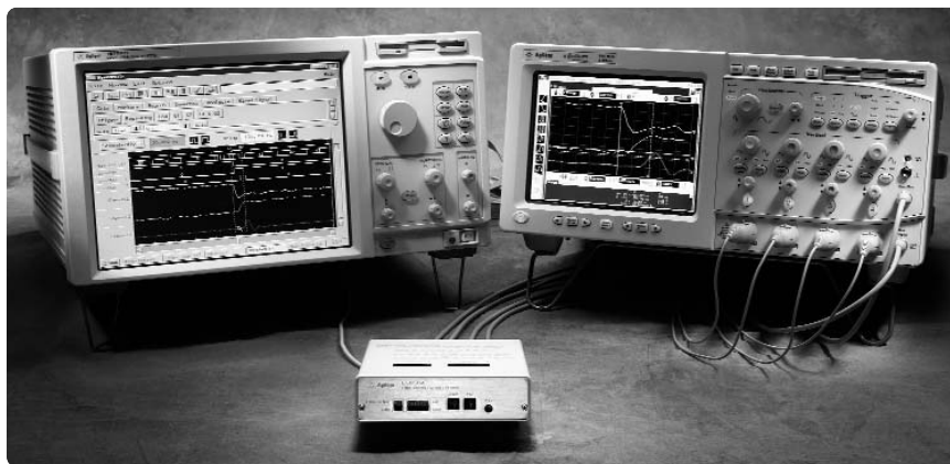
Figure 10.1. Agilent E5850A time-correlation fixture bridges the analog and digital worlds to track down problems more quickly.
