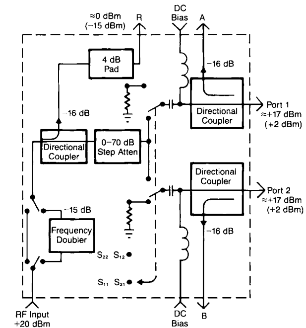
HP 85047A Schematic
