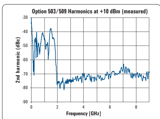
Harmonics (measured)
