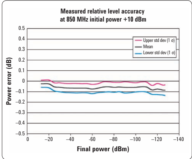
Relative level accuracy measures the accuracy of a step change from any power level to any other power level. This is useful for large changes (such as 5 dB steps).
