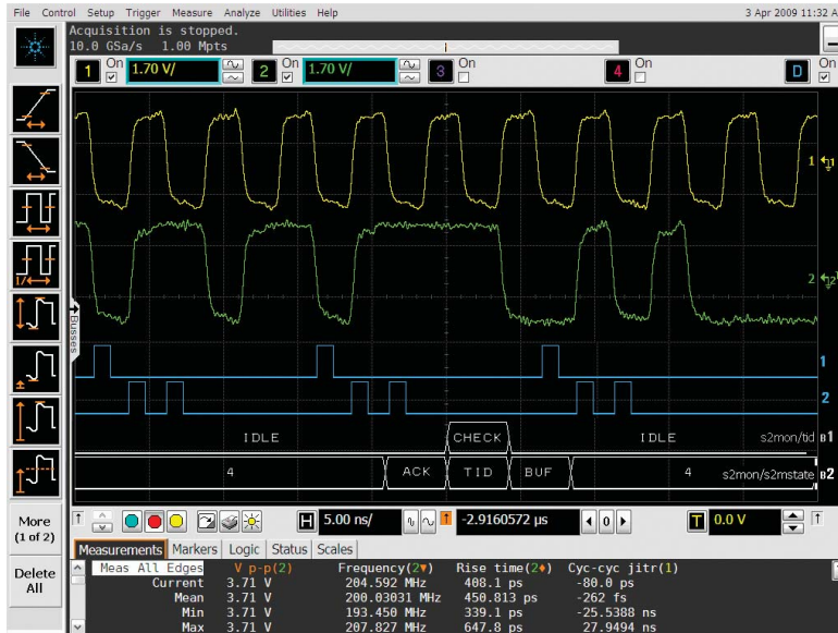
Use the MSO timing channels to evaluate control signal relationships and data buses up to 16 bits wide. Use symbols to more quickly interpret waveforms.
