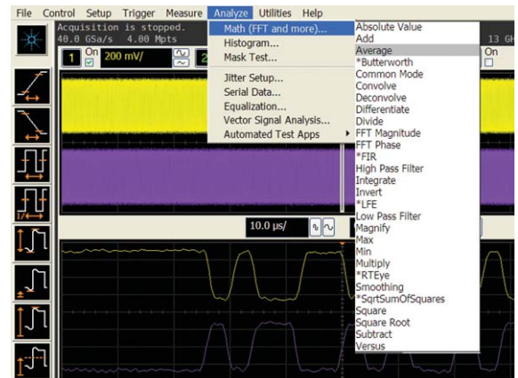
Mask tests, histograms and a wide variety of functions provide deep signal analysis.
