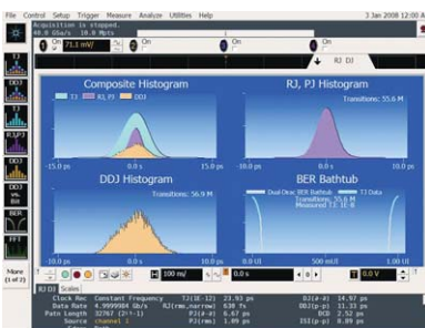
Analyze jitter plus RJ/DJ separation.
