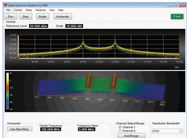
Waterfall view for ASV spectrogram measurement
