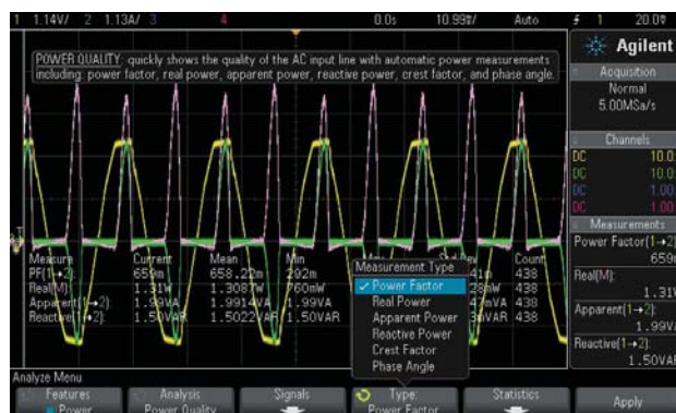
An example screen for power quality analysis
