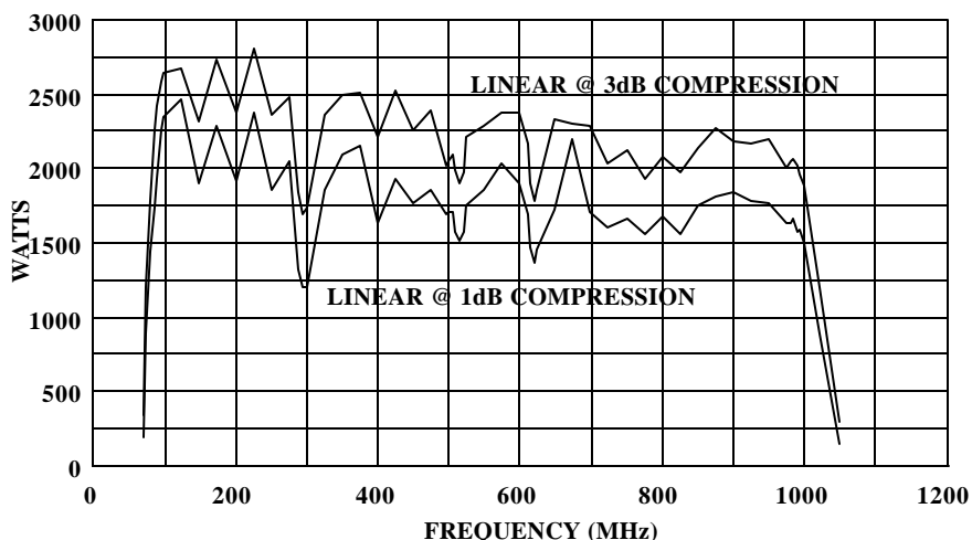
2000W1000A TYPICAL POWER OUTPUT
