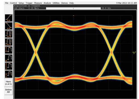
10 Gbps eye captured with 20 GHz of bandwidth
