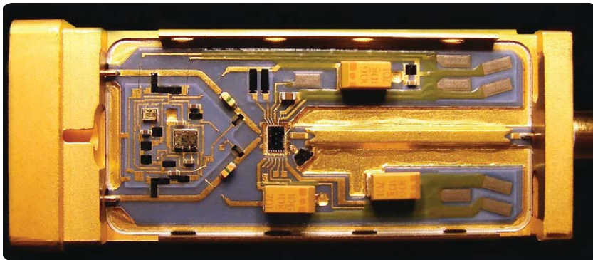
The InfiniiMax III probing system uses the same InP technology that enables high bandwidth and low noise oscilloscope measurements.
