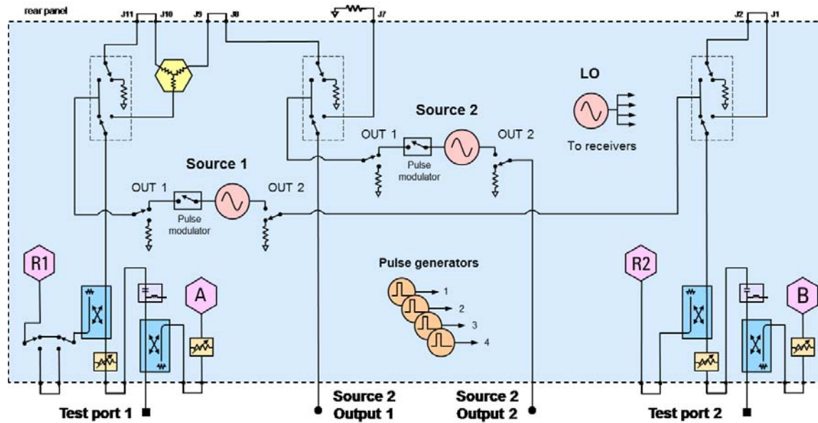
Figure 4. 2-Port N5244A and N5245A Option 224 with 029
