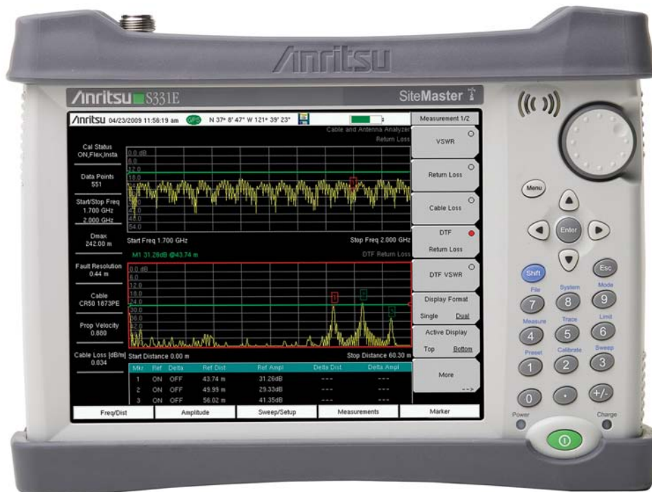
Site Master™ S331E Cable & Antenna Analyzer featuring 8.4 inch Daylight Viewable Touchscreen Compact Size: 273 mm x 199 mm x 91 mm (10.7 inch x 7.8 inch x 3.6 inch), Lightweight: 2.71 kg (6.0 lbs)
