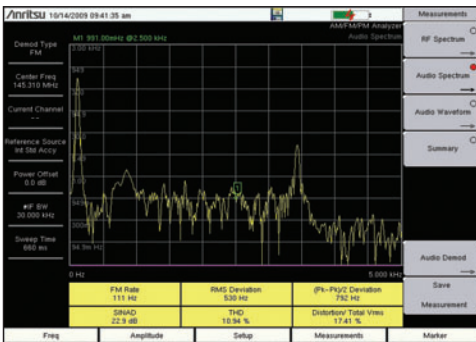
AM/FM/PM Analyzer
