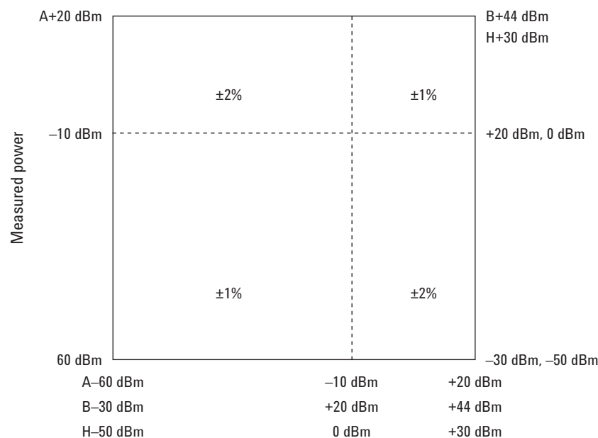
Figure 2. Relative mode power measurement linearity with an EPM Series power meter, at 25^{\circ}\text{C} \pm 10^{\circ}\text{C} (typical)
