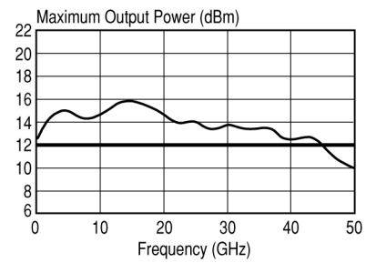
83051A Amplifier
