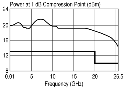
83006A Amplifier
