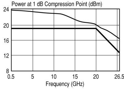
83017A Amplifier
