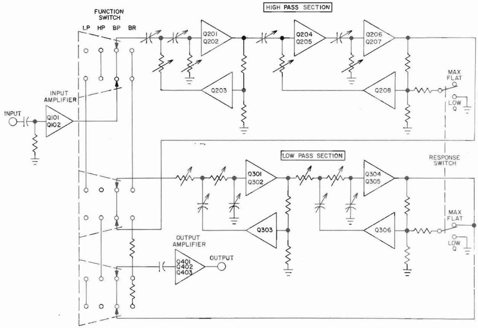
Figure 4-1. Block Diagram
