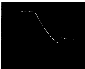
Figure 2A. Data taken on network analyzer using multiplier-type oscillators. By-products of multiplied frequencies give erroneous indication of response outside filter passband.
