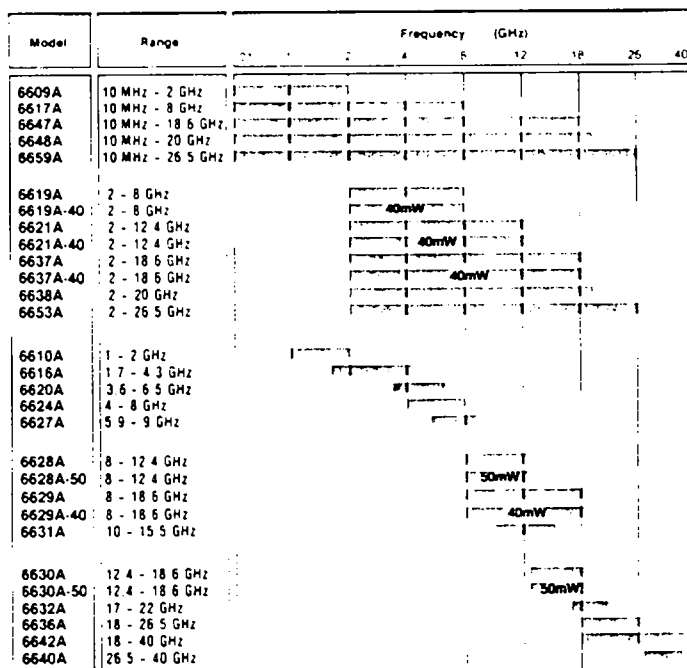
Figure 1. The 6600A Programmable Sweep Generator family covers the 10 MHz to 40 GHz range.
