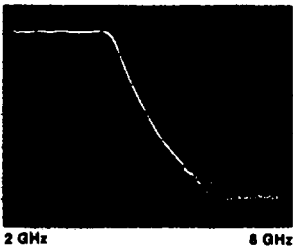
Figure 2B. Data taken with WILTRON Network Analyzer. Clean signals from fundamental oscillators show that response outside passband is actually 20 dB less than shown in 2A.
