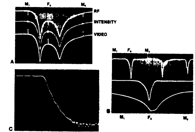
Figure 4. (A) F_0 , M_1 , M_2 markers are displayed as RF, intensity, or video pips. (B) In F_0 - F_2 sweep (top), M_1 and M_2 markers can be used to select limits of M_1 - M_2 sweep (center). The F_0/\Delta F sweep (bottom) with M_1 , M_2 markers sweeps symmetrically about F_0 from 0 to 100% of full band. (C) When used with the 560A Network Analyzer, the 6600A markers can be tilted for optimum display on vertical traces.
