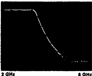
Figure 2B. Data taken with WILTRON Network Analyzer. Clean signals from fundamental oscillators show that response outside passband is actually 20 dB less than shown in 2A.
