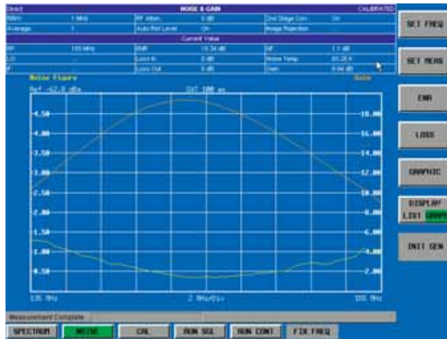
Noise figure measurement with Noise Measurement Software R&S®FS-K30.
