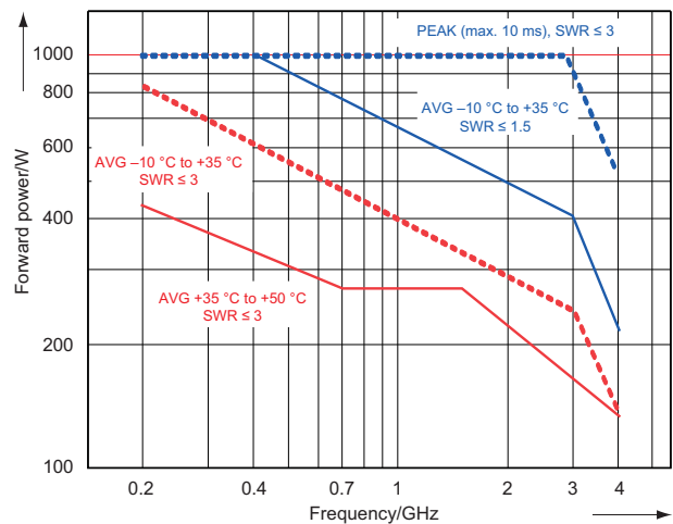
Power-handling capacity
