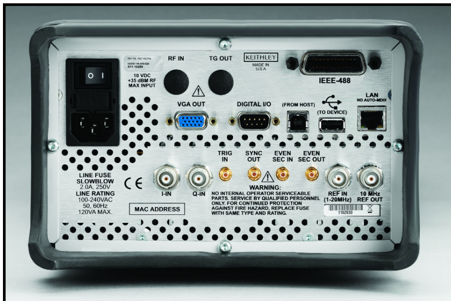
Model 2810 rear panel.
