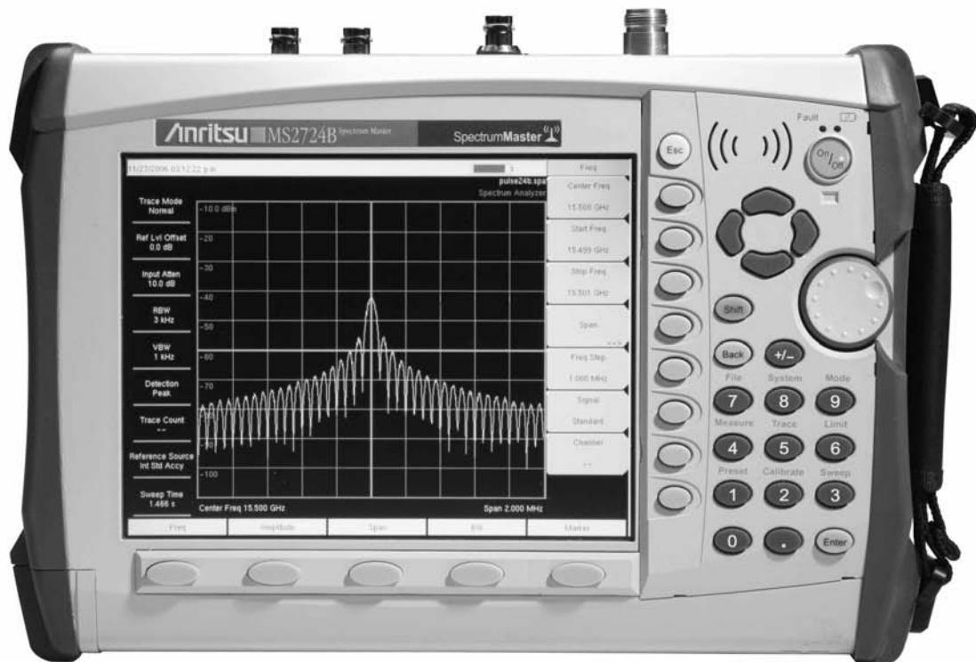
The Anritsu MS2724B is the most advanced ultra-portable spectrum analyzer on the market, featuring unparalleled performance at a modest price.
