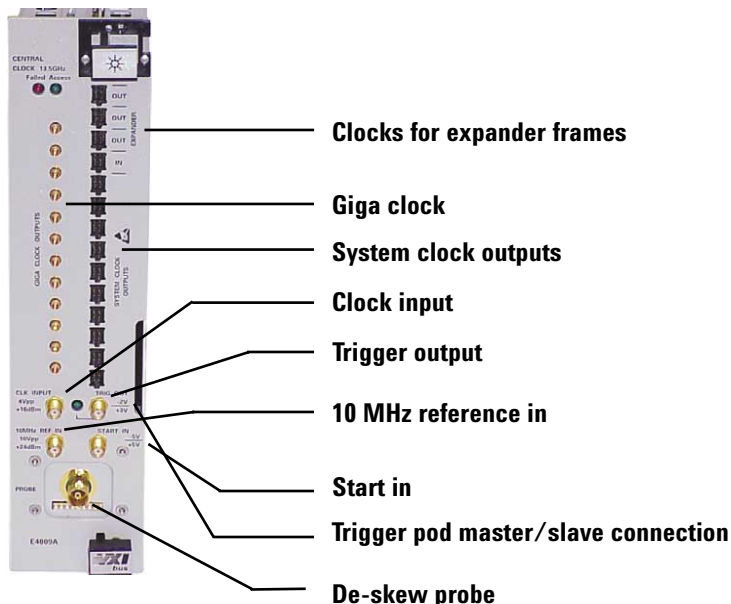
Figure 31. E4809A module
