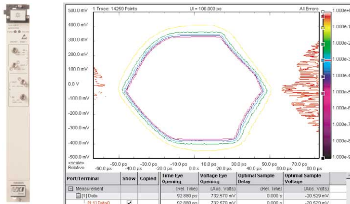
Figure 21. E4867A analyzer with eye diagram
