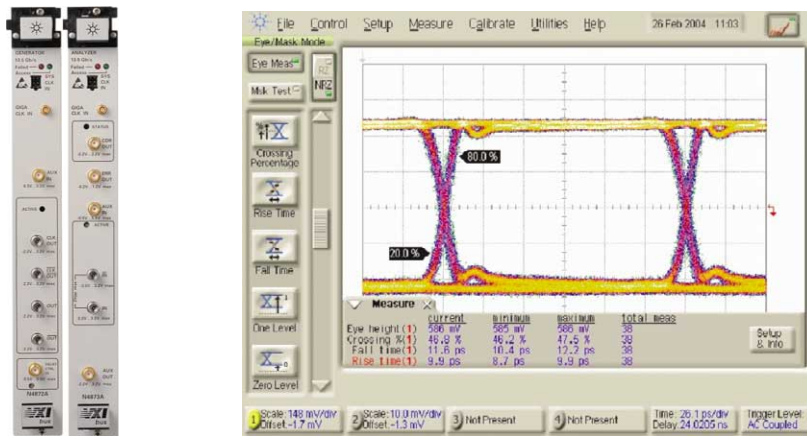
Figure 22. N4874A & N4875A and waveform
