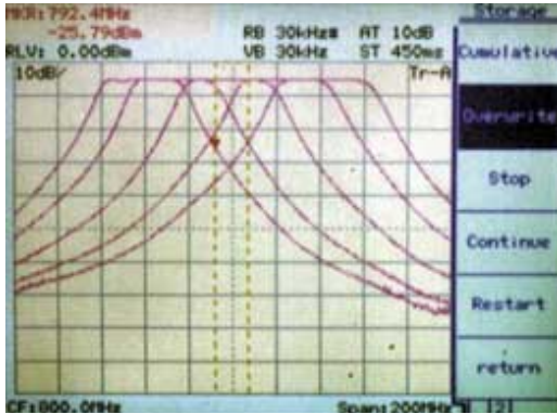
Bandpass filter adjustment
