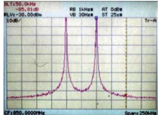
Two-signal third order intermodulation
