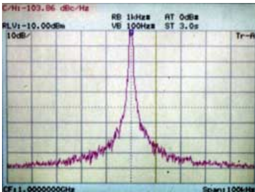
Noise sidebands measurement (10 kHz offset)
