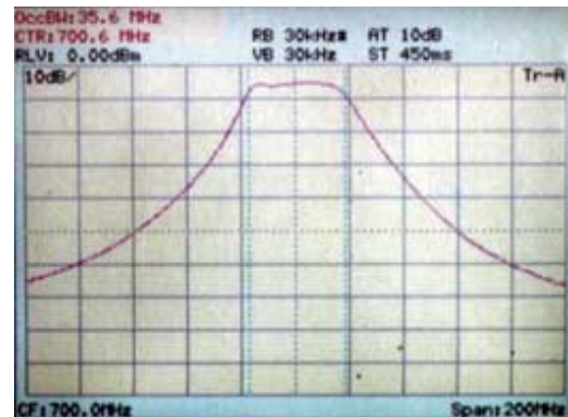
Bandpass filter measurement
