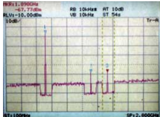
Multi-zone sweep
