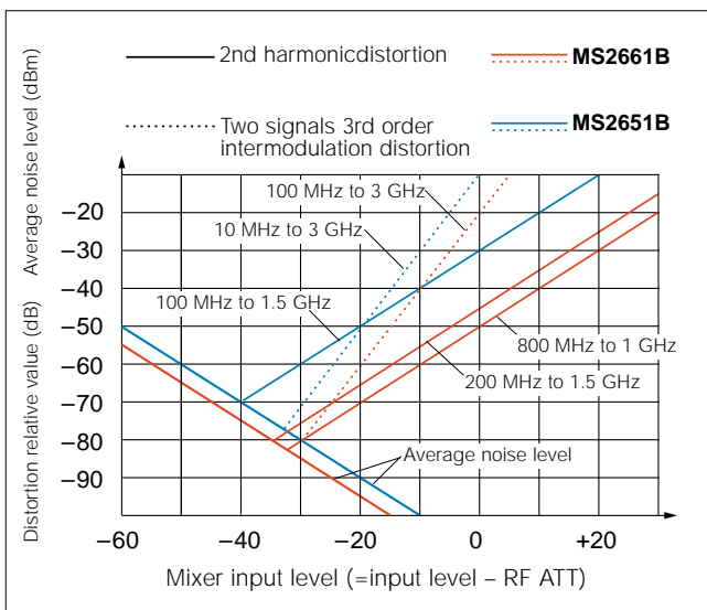
Distortion characteristics
