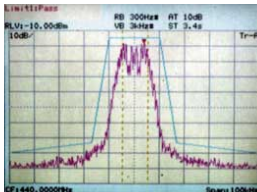
Mask measurement
