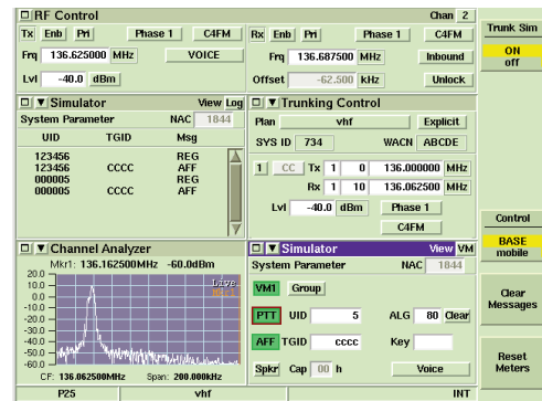
P25 Trunking Simulation with Virtual Mobile
