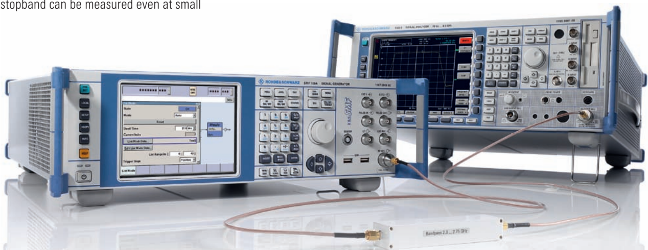
Scalar network analysis with the R&S®SMF100A microwave signal generator and the R&S®FSP-B10 spectrum analyzer with the R&S®FSP-B10 option installed
