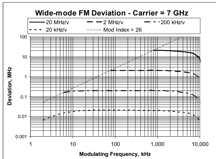
Wide-mode deviation as a function of modulating frequency at 1 V Peak Input (Supplemental)
