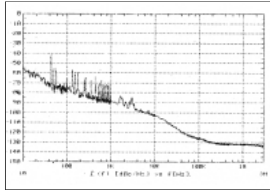
SSB phase noise at 1.9 GHz
