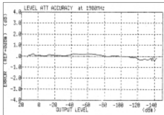
Output level accuracy at 1.9 GHz
