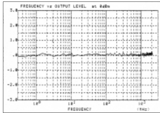
Output level frequency characteristics
