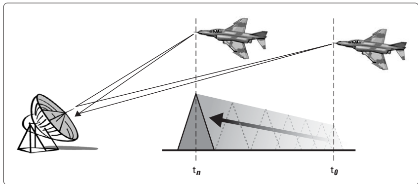
Figure 3. Closing targets can be simulated by ranging parameters on each pulse.
