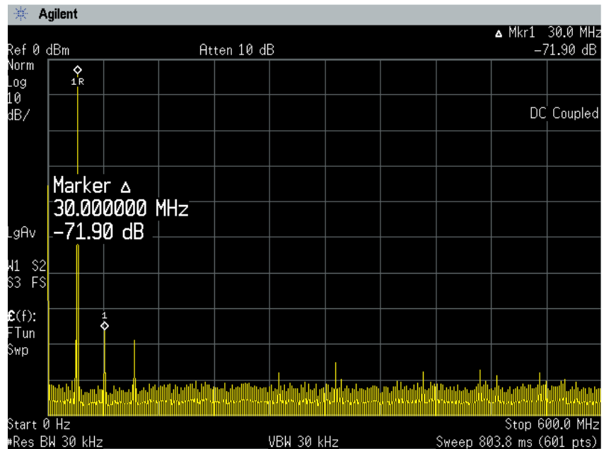
Figure 8. Spurious performance outstanding at low signal frequencies.
