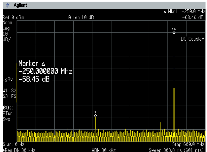
Figure 7. Excellent harmonic and spurious performance are available across the fullbandwidth of each channel.
