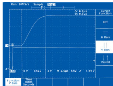
Rise and fall times of only a few µs can be reached under all load conditions that comply with the R&S® NGPX specifications
