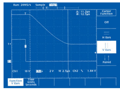
Rise and fall times of only a few µs can be reached under all load conditions that comply with the R&S® NGPX specifications
