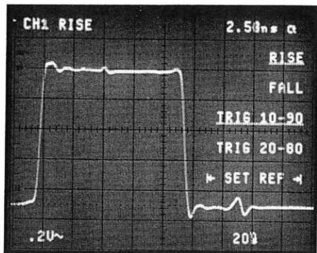
Make difficult measurements faster and more accurately. Rise time measurements are made automatically with the integrated 200 MHz counter/timer on the 2247A and 2252.
