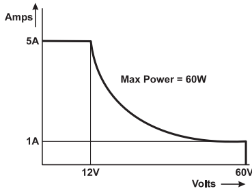
Autorangeing Curve for 60 V/5 A/60 W Power Module
