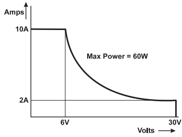
Autorangeing Curve for 30 V/10 A/60 W Power Module
