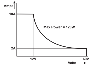
Autorangeing Curve for 60 V/10 A/120 W Power Module
