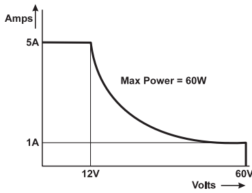
Autorange Curve for 60 V/5 A/60 W Power Module
