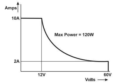
Autorange Curve for 60 V/10 A/120 W Power Module
