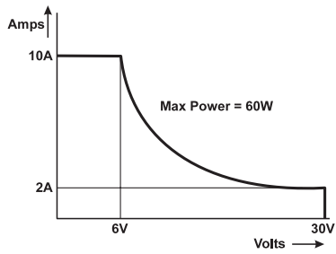
Autorange Curve for 30 V/10 A/60 W Power Module
