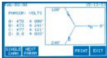
Meter Mode A true three-phase volt-ampere-power-harmonic meter lets you view values updated every second. ■ V, A, W, VA, VAR, power factor, frequency, voltage unbalance, voltage and current THD, current crest factor, K factor, demand, energy and individual harmonics ■ voltage and current phasor diagrams
