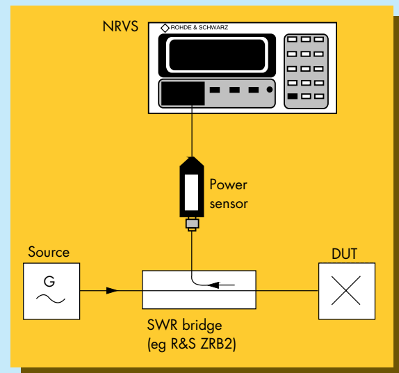
Thanks to their wide dynamic range, the NRVS power sensors are ideal for measuring small reflection coefficients, eg by using SWR Bridge ZRB2.
