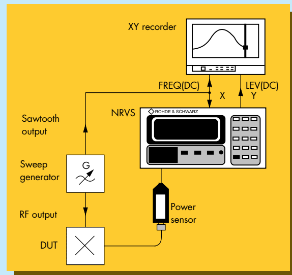
This setup is used for measuring and recording the powertransfer characteristic of a DUT.
