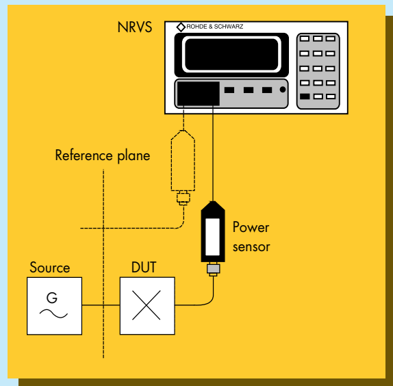
Depending on the measuring head used, attenuations of up to 90 dB can be measured with the NRVS.
