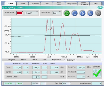
40 Gb/s modulation with CS-RZ, PSBT-NRZ, and DPSK-RZ modulation schemes
