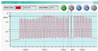
46 channel DWDM spectrum
