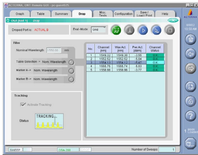
Channel drop/isolation function
