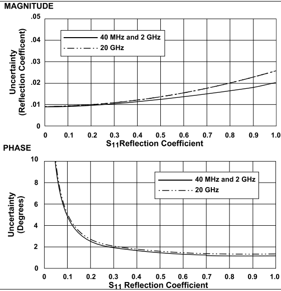
Models 37225A and 37247A (GPC-7 Connectors), Reflection Measurements
