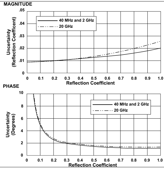
Models 37225A and 37247A (K Connectors), Reflection Measurements
