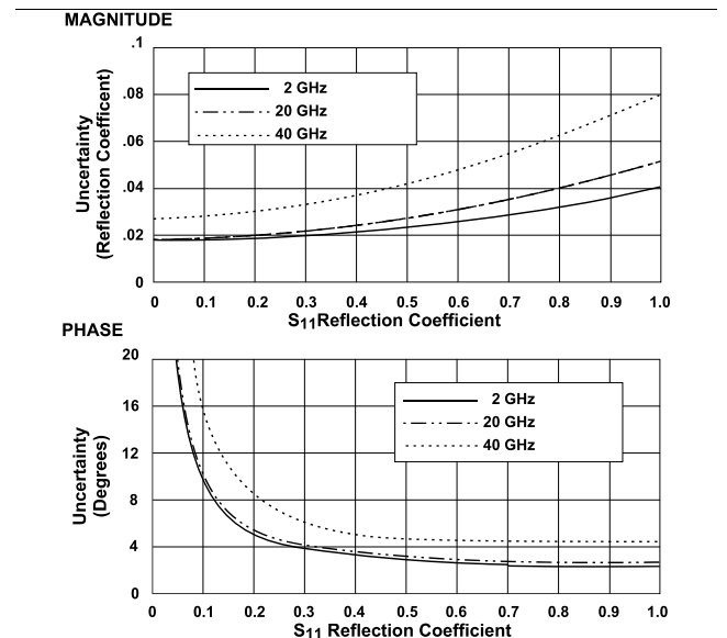
Model 37269A Universal Test Fixture (Model 3680K), Microstrip LRL Calibration (Model 36804-10, 10 mil Calibration Kit — Reflection Measurements
