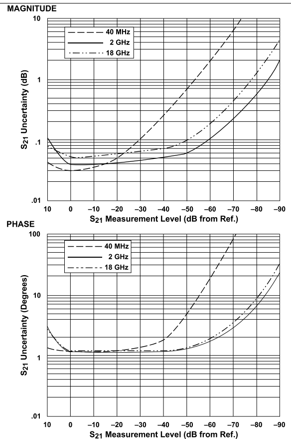
Models 37225A and 37247A (Type N Connectors), Transmission Measurements
