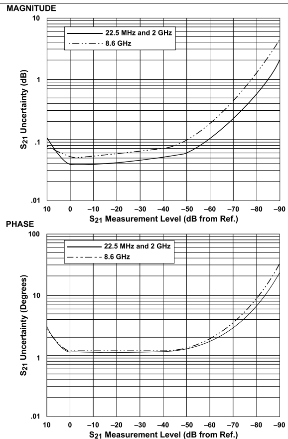
Models 37211A and 37217A (Type N Connectors) Transmission Measurements
