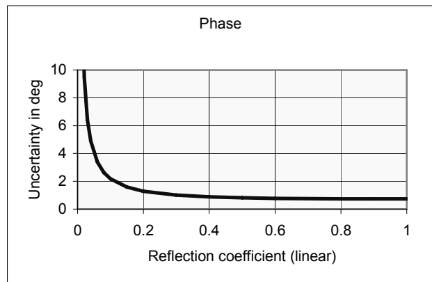
Typical accuracy of reflection magnitude and reflection phase measurements of R&S®ZVB4 in the frequency range from 300 kHz to 4 GHz, of R&S®ZVB8 in the frequency range from 300 kHz to 8 GHz, and of R&S®ZVB20 in the frequency range from 50 MHz to 20 GHz
