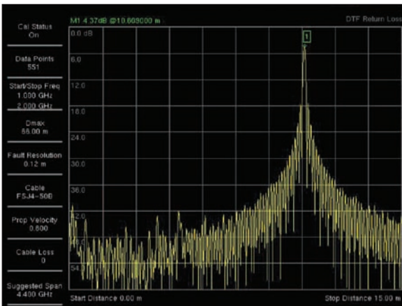
Distance-To-Fault
