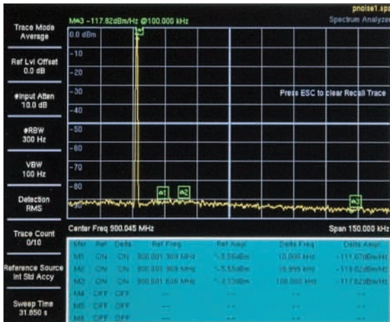
Phase Noise
