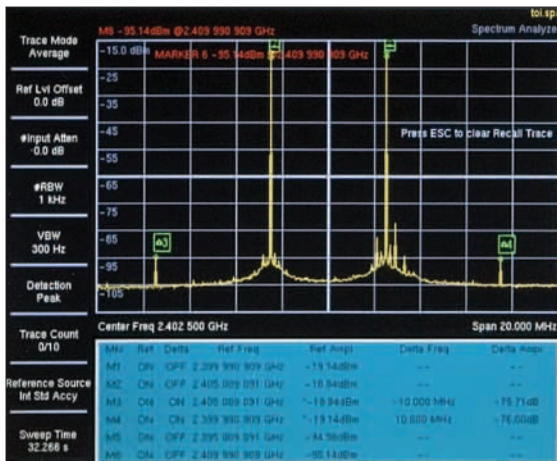
Signal Measurements
