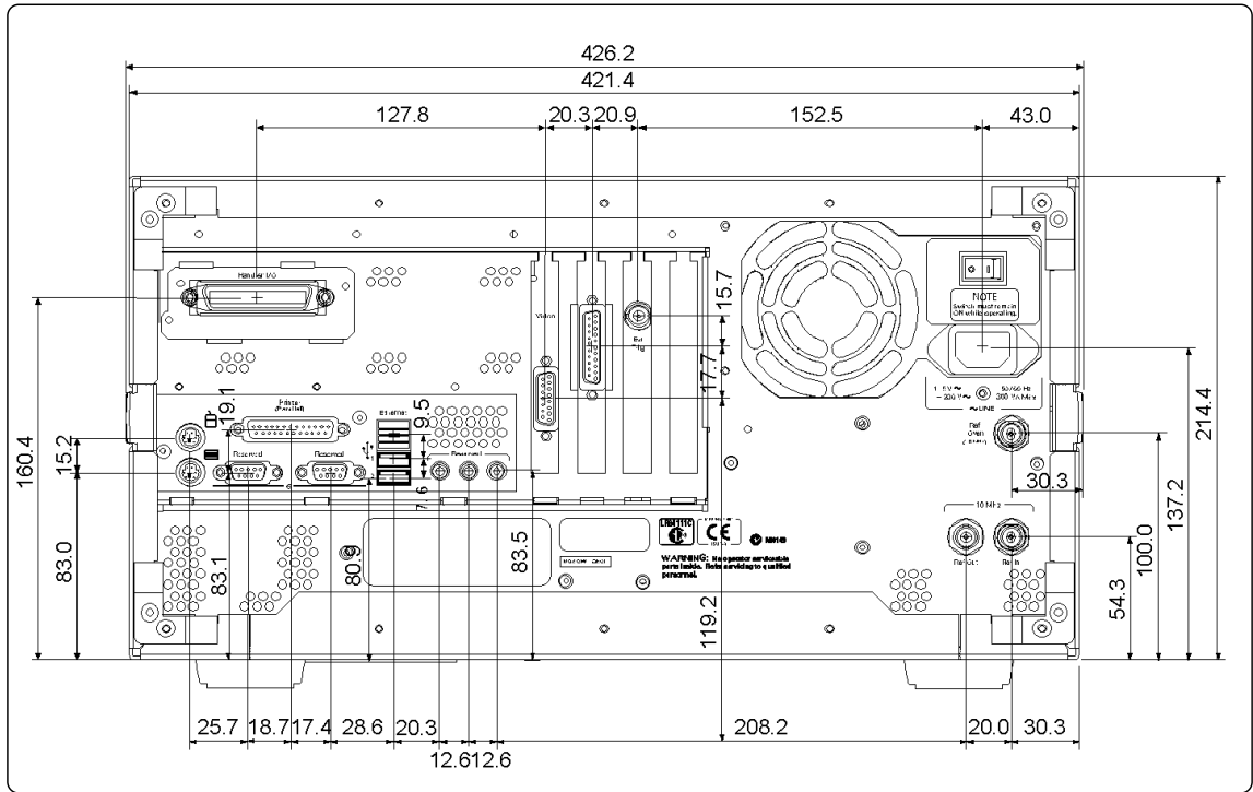
Figure 1-2. Dimensions (rear view, with option E5070B/E5071B-1E5, in millimeters, nominal)
