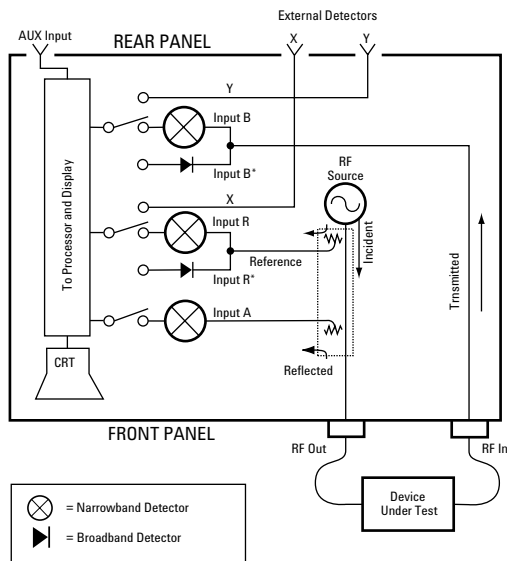
8712B/8713B block diagram
