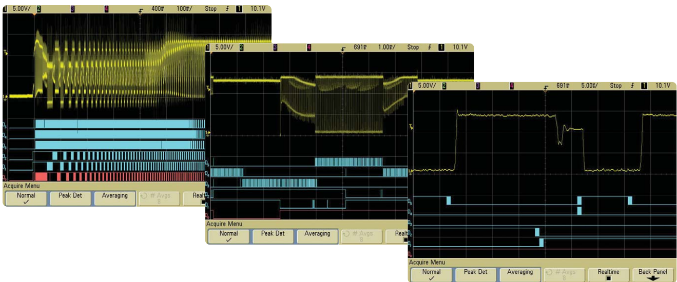
Figure 3. Motor drive signal start-up sequence with digital control signal triggering and various levels of zoom reveal "runt" pulse using Agilent's MSO6000A Series MSOs.
