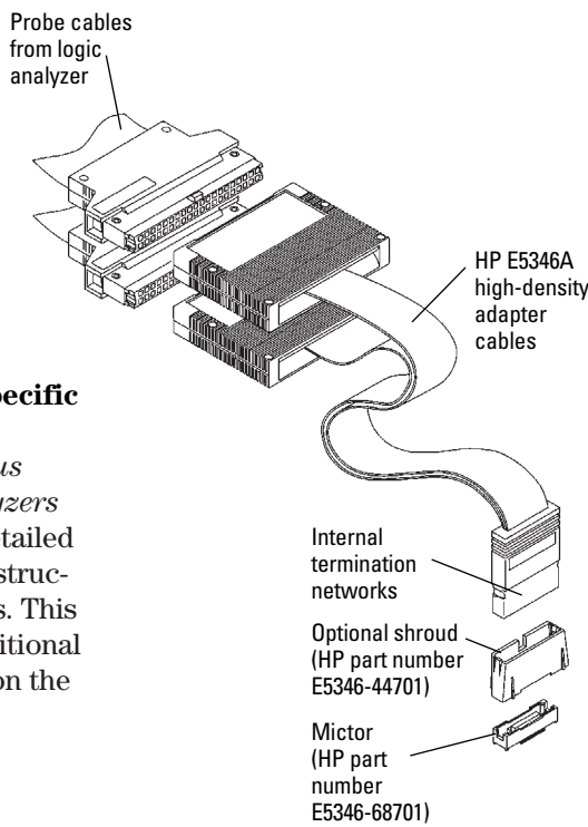
Figure 9. High density direct connection solution
