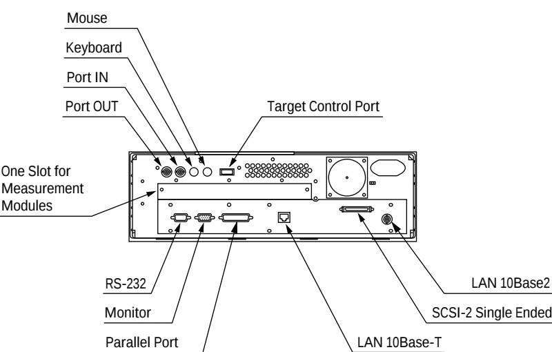
Figure 17. HP 16600A Series rear panel
