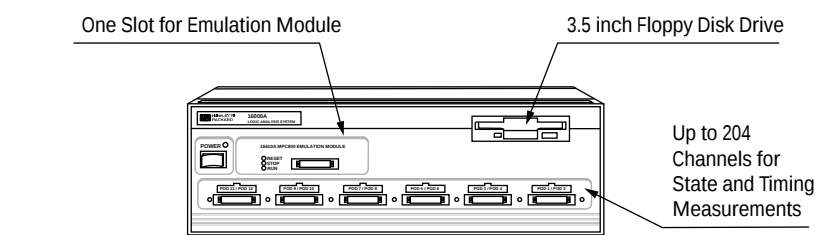
Figure 16. HP 16600A Series front panel
