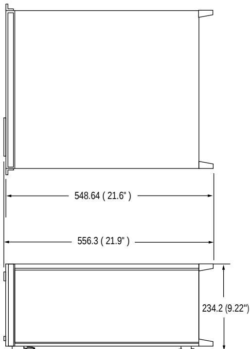
Figure 21. HP 16700A, 16701A and 16702A exterior dimensions. Dimensions: mm (inches).
