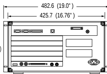
Figure 21. HP 16700A, 16701A and 16702A exterior dimensions. Dimensions: mm (inches).
