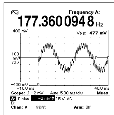
Figure 5b. By comparison, this figure shows how too high a sensitivity in a traditional counter could give erroneous results. Too high a trigger sensitivity means that noise forces the input signal to cross the trigger level (very narrow hysteresis band) more than once per input cycle and cause false counts.
