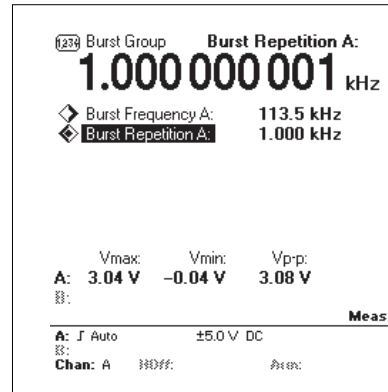
Figure 7b. The MultiFunction Counter measures automatically and shows simultaneously both the burst frequency and the burst repetition frequency.
