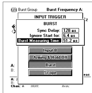
Figure 7c. The Burst settings, as automatically derived from the input signal (in figures 4a and 4b) by the green AUTO SET button.
