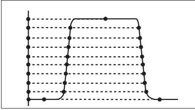
Figure 1a. This drawing shows how the MultiFunction Counter's unique Transitional-sampling™ concentrates sample data on transitions, obtaining a high time resolution of <1ns in all time base positions (>1 GSa/s effective sample rate).
