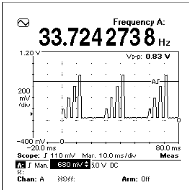
Figure 6a. Frequency measurement with manual trigger level setting, where only the last pulse in each pulse-burst triggers the counter. This means you can measure the repetition frequency of the burst reliably.
