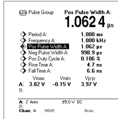
Figure 2c. In the VALUES presentation mode, all signal parameters can be shown simultaneously, without the need for setting changes per measurement. Any parameter can be selected as "primary", to be displayed at the top of the screen in large numerals and with full resolution.
