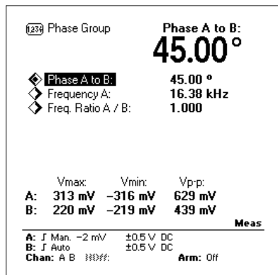
Figure 3b. The Vp-p values of the output and input signals indicate a ratio of 439mV \div 629mV = 0.7 i.e. at the frequency where the output signal B is 3dB down versus the input signal A. The frequency and the phase delay are measured simultaneously with high accuracy.
