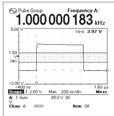
Figure 2b. This screen shows all the pulse details yet is 1000 x faster than in figure 2a. Simultaneously the frequency is measured with 10 digits resolution.
