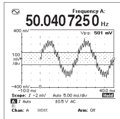
Figure 5a. The MultiFunction Counter gives correct results even on a noisy signal. AUTO Trigger centers the trigger level at 50% of amplitude and adjusts the trigger hysteresis band (noise immunity band) to 33% of the input amplitude to provide optimal noise immunity.
