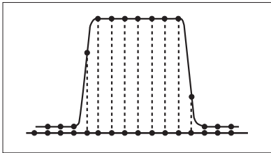
Figure 1b. By comparison, this drawing shows Time Sequential sampling, which is traditionally used in DSOs. Only a few samples are taken on transitions, creating the risk that very narrow pulses will be missed.
