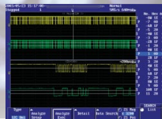
Analysis results of 6.4 seconds of I 2 C data.
