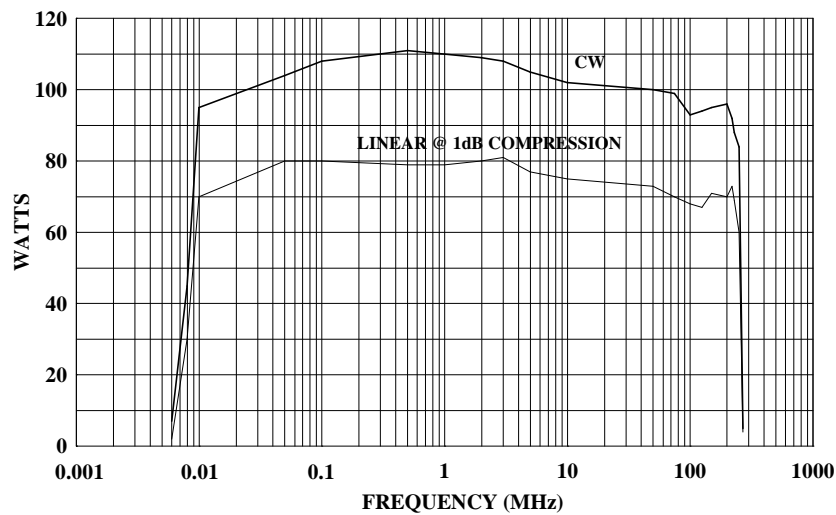
75A250 TYPICAL POWER OUTPUT
